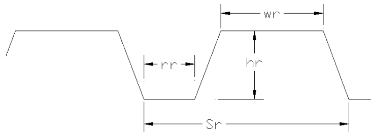
Figure 170: Deck dimension parameters
