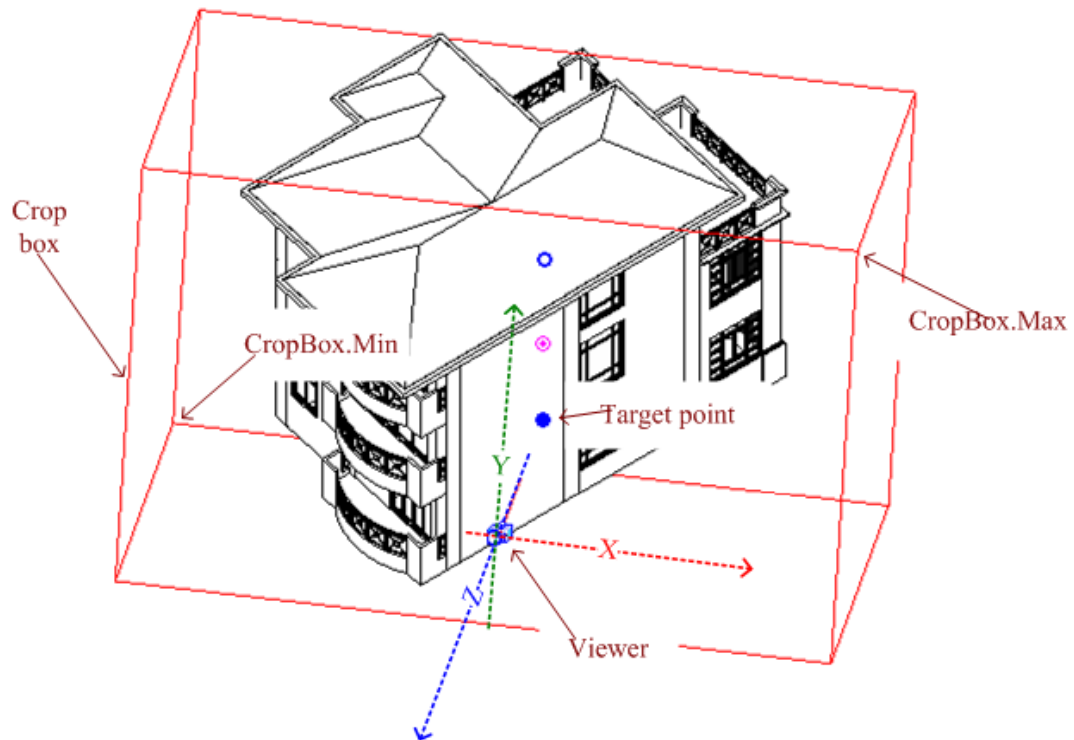
Figure 98: Parallel projection
