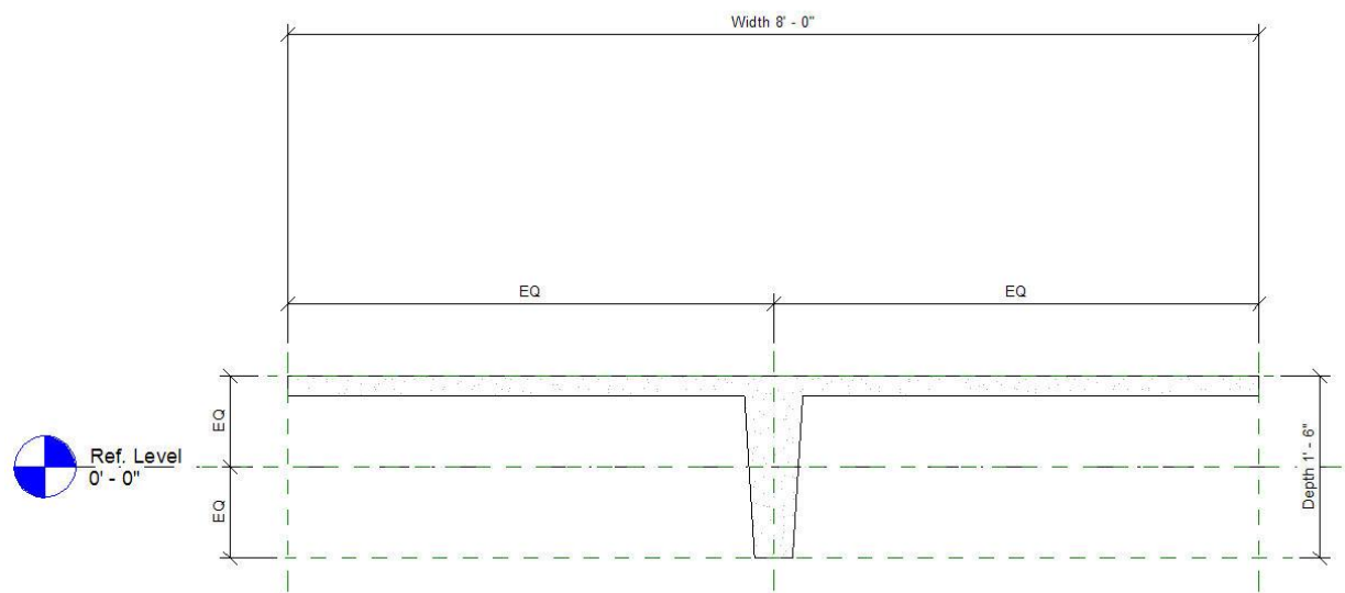
Figure 189: Precast-Single Tee Cross Section 2
