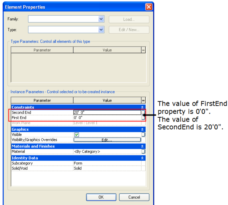
Figure 85: Blend parameters in the UI
