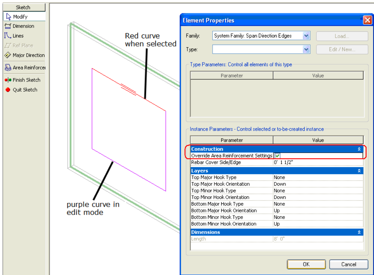
Figure 154: AreaReinforcementCurve in edit mode
