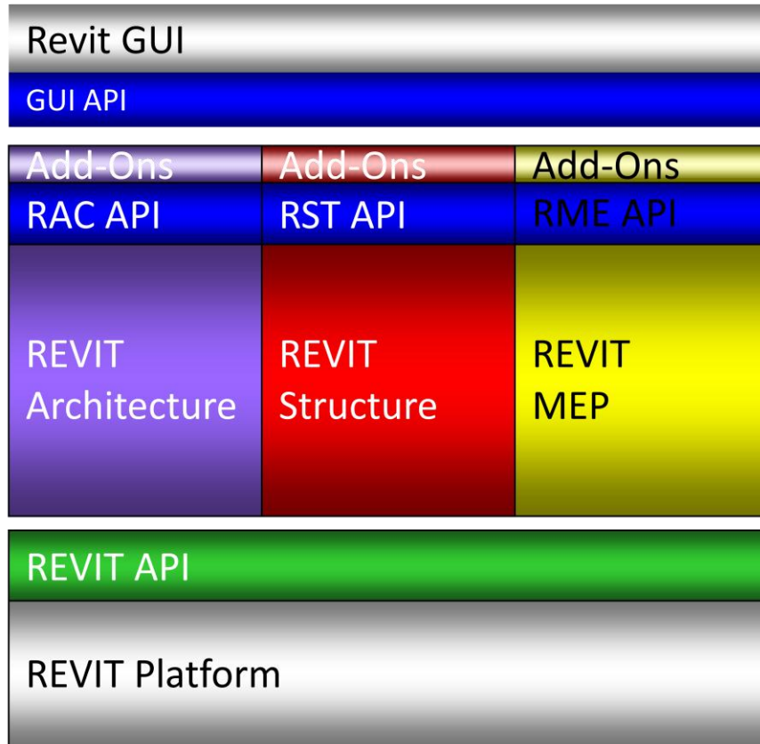
Figure 11: Revit, RevitAPI and Add-ins
