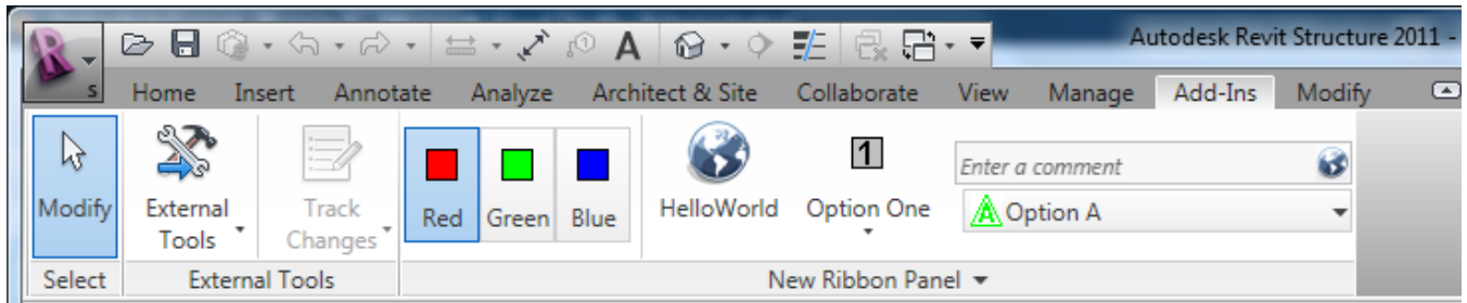
Figure 14: New ribbon panel and controls
