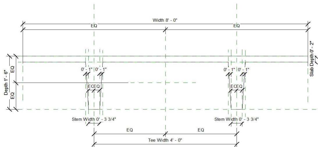
Figure 195: Precast-Double Tee Cross Section
