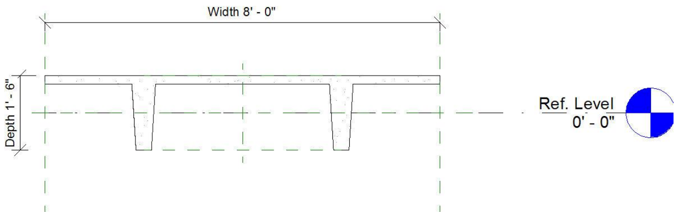
Figure 196: Precast-Double Tee Cross Section 2
