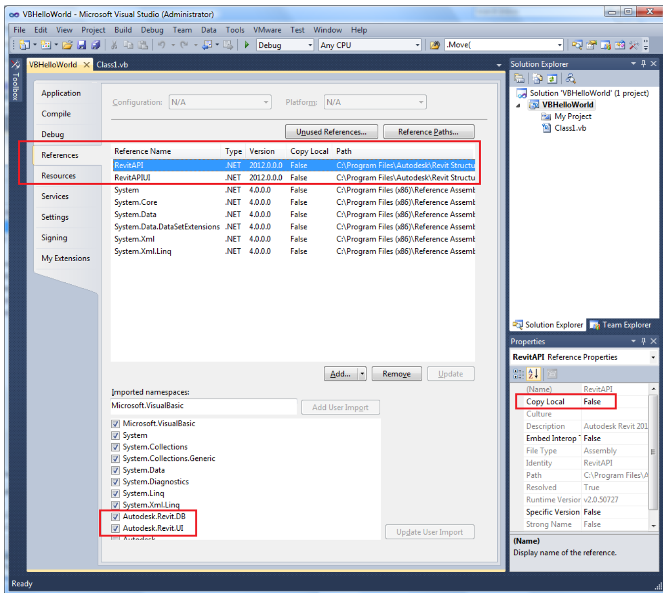
Figure 173: Add references and import Namespaces
