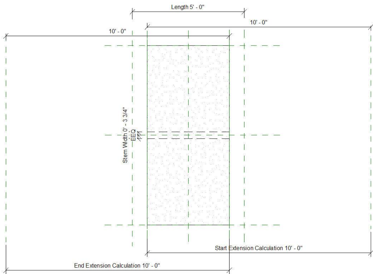
Figure 189: Precast-Single Tee Cross Section 2
