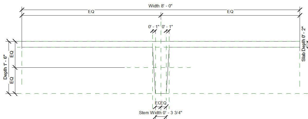
Figure 188: Precast-Single Tee Cross Section
