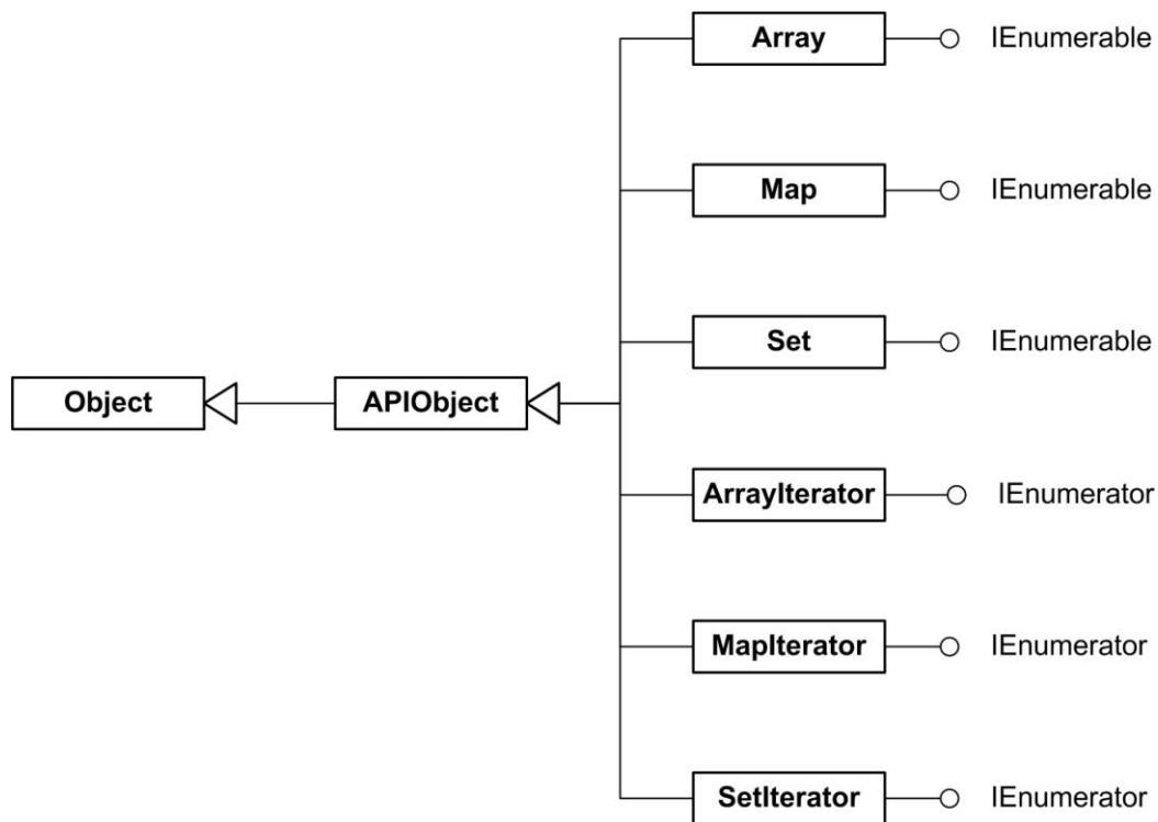
Figure 36: Collection diagram
