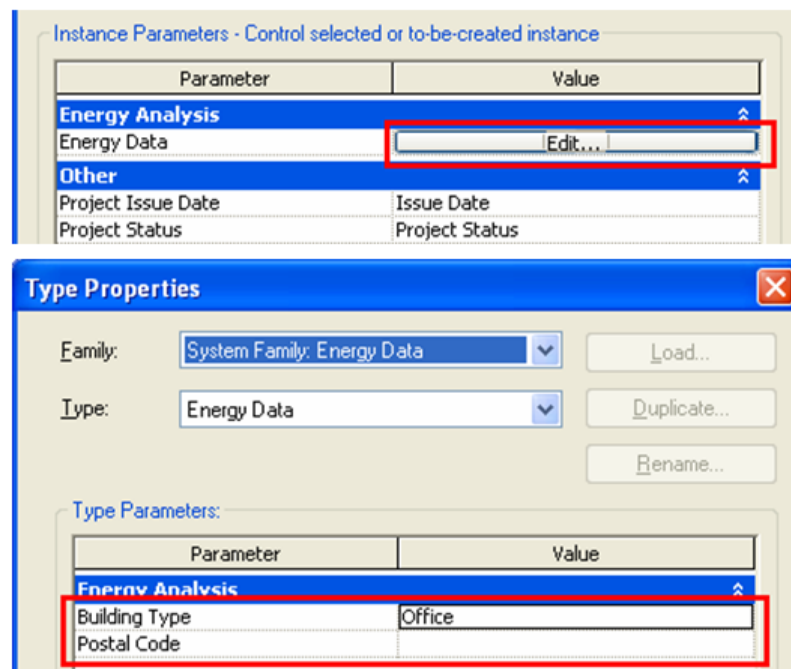
Figure 173: gbXMLParamElem setting
