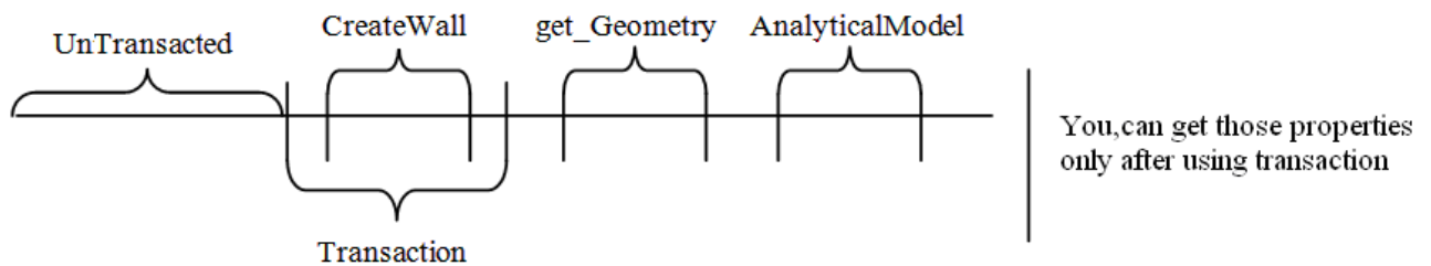
Figure 156: Transaction timeline
