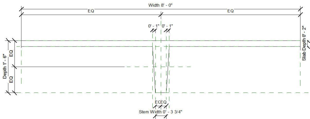
Figure 204: Precast-Single Tee Cross Section
