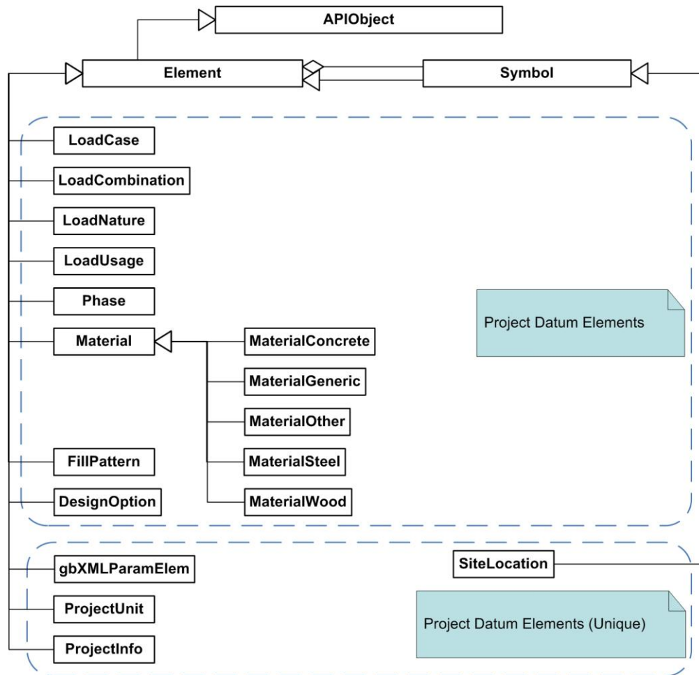
Figure 67: Information Elements diagram
