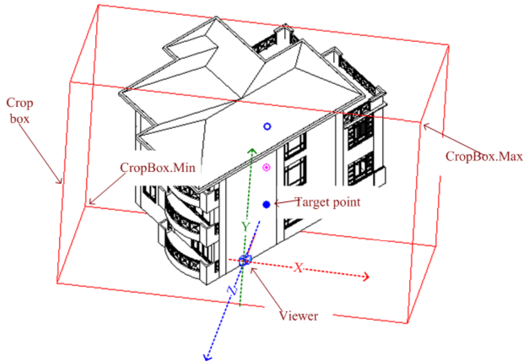
Figure 107: Parallel projection
