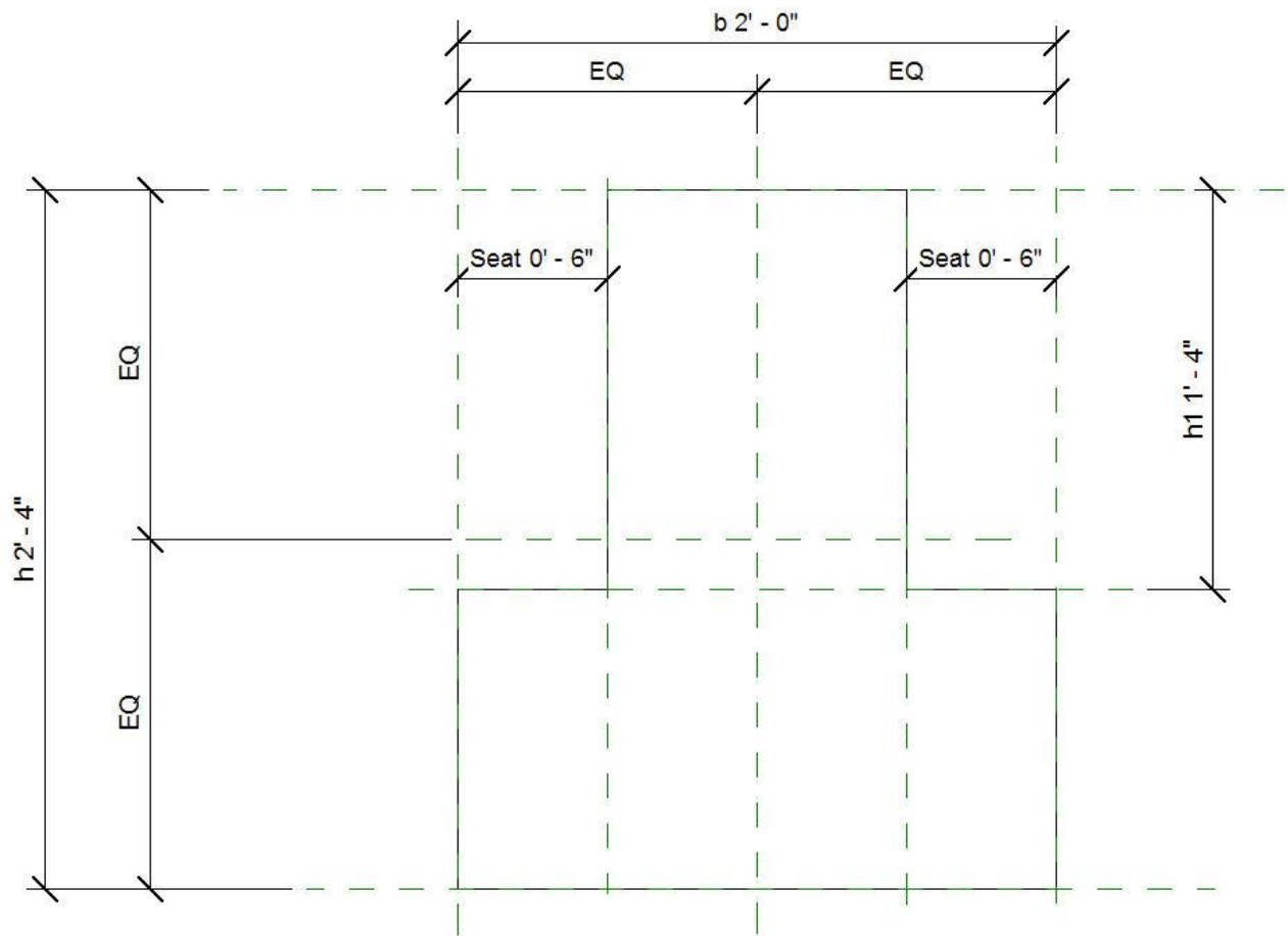
Figure 208: : Precast-Inverted Tee Cross Section
