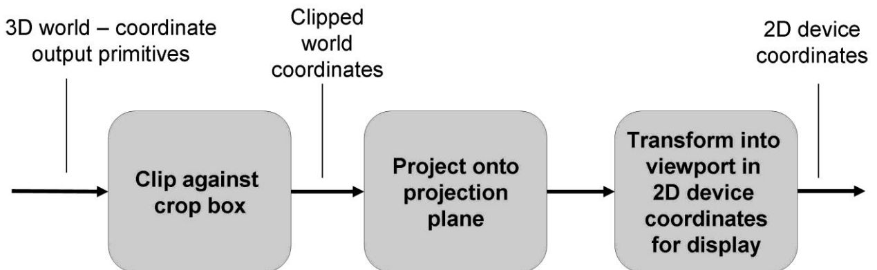
Figure 102: Create view process
