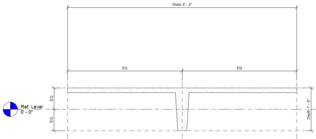
Figure 205: Precast-Single Tee Cross Section 2
