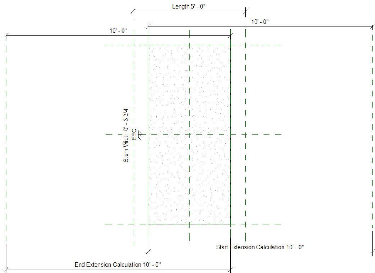
Figure 205: Precast-Single Tee Cross Section 2
