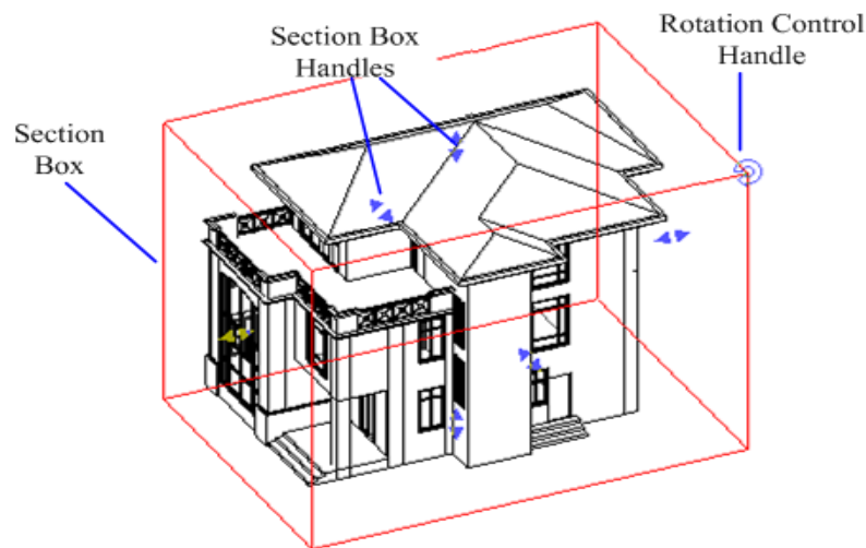
Figure 109: Section box
