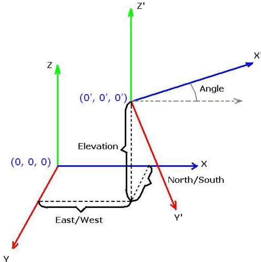
Figure 144: Geographical offset and rotation sketch map
