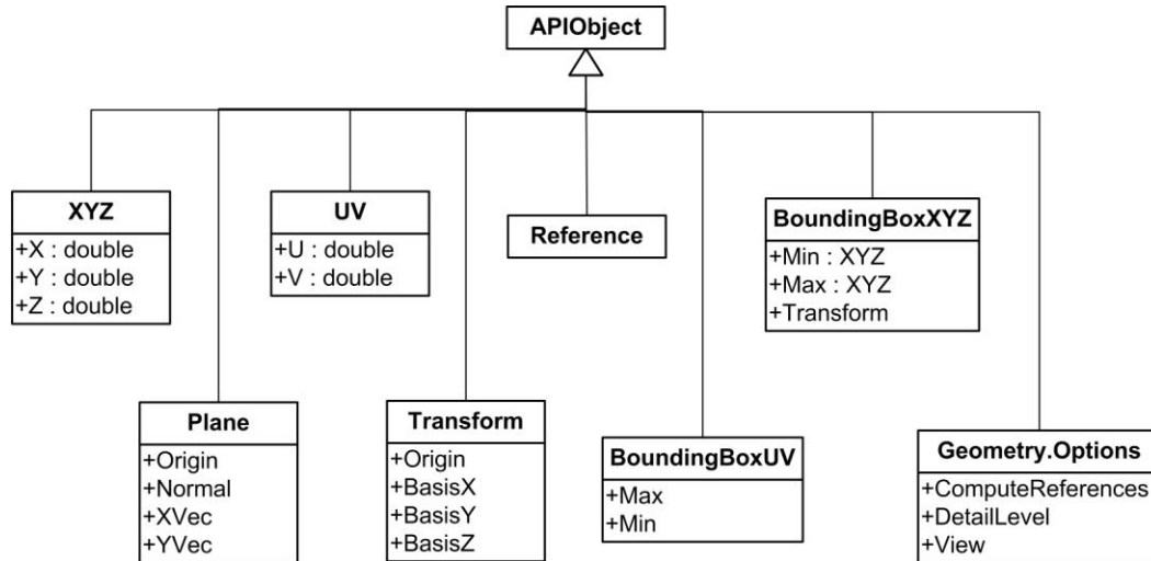
Figure 127: Geometry helper hierarchy diagram
