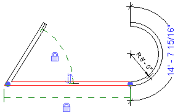
Figure 74: Linear and Radial dimension constraints
