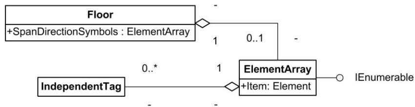
Figure 178: SpanDirectionSymbols diagram
