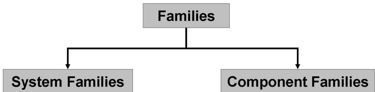
Figure 24: Families
