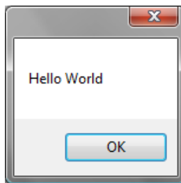
Figure 5: System message
