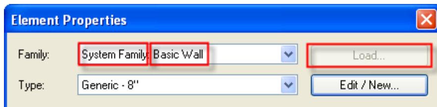
Figure 52: System Family
