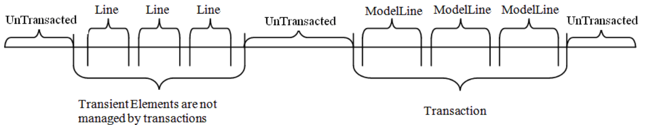
Figure 155: Transaction timeline
