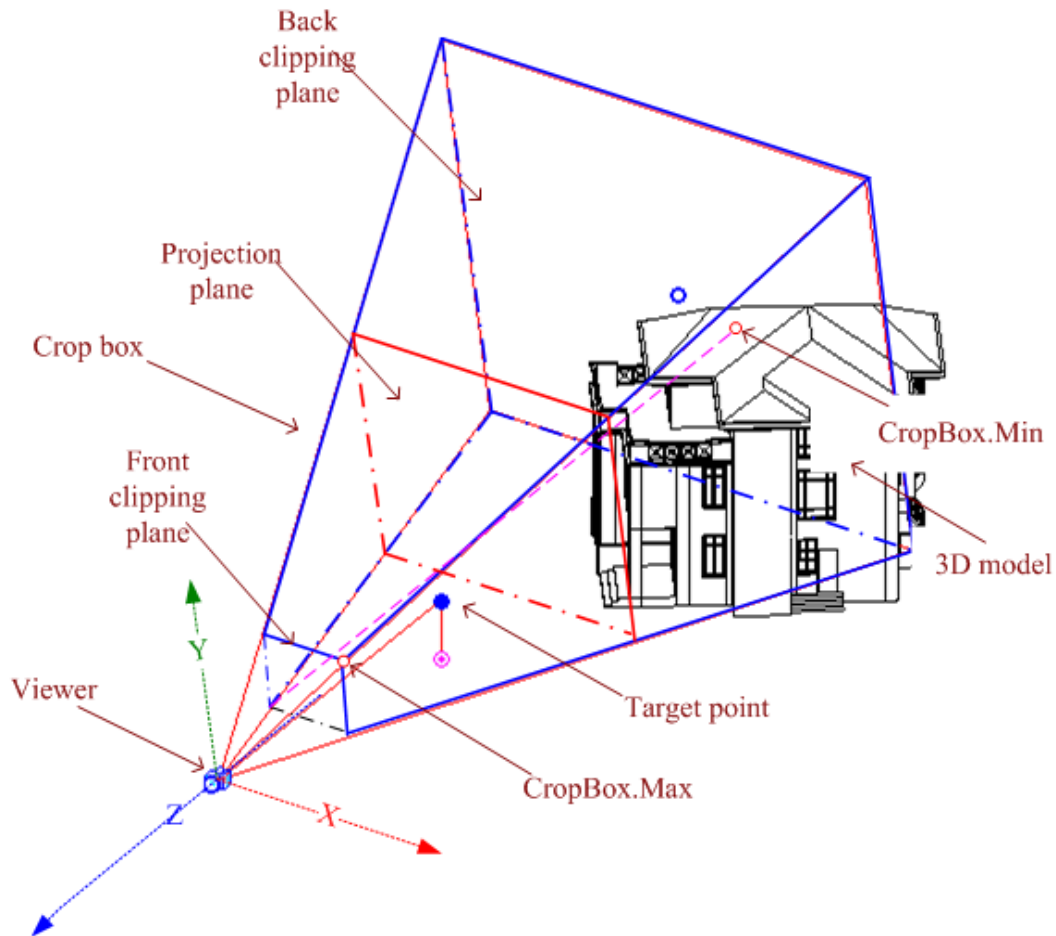
Figure 105: Perspective projection
