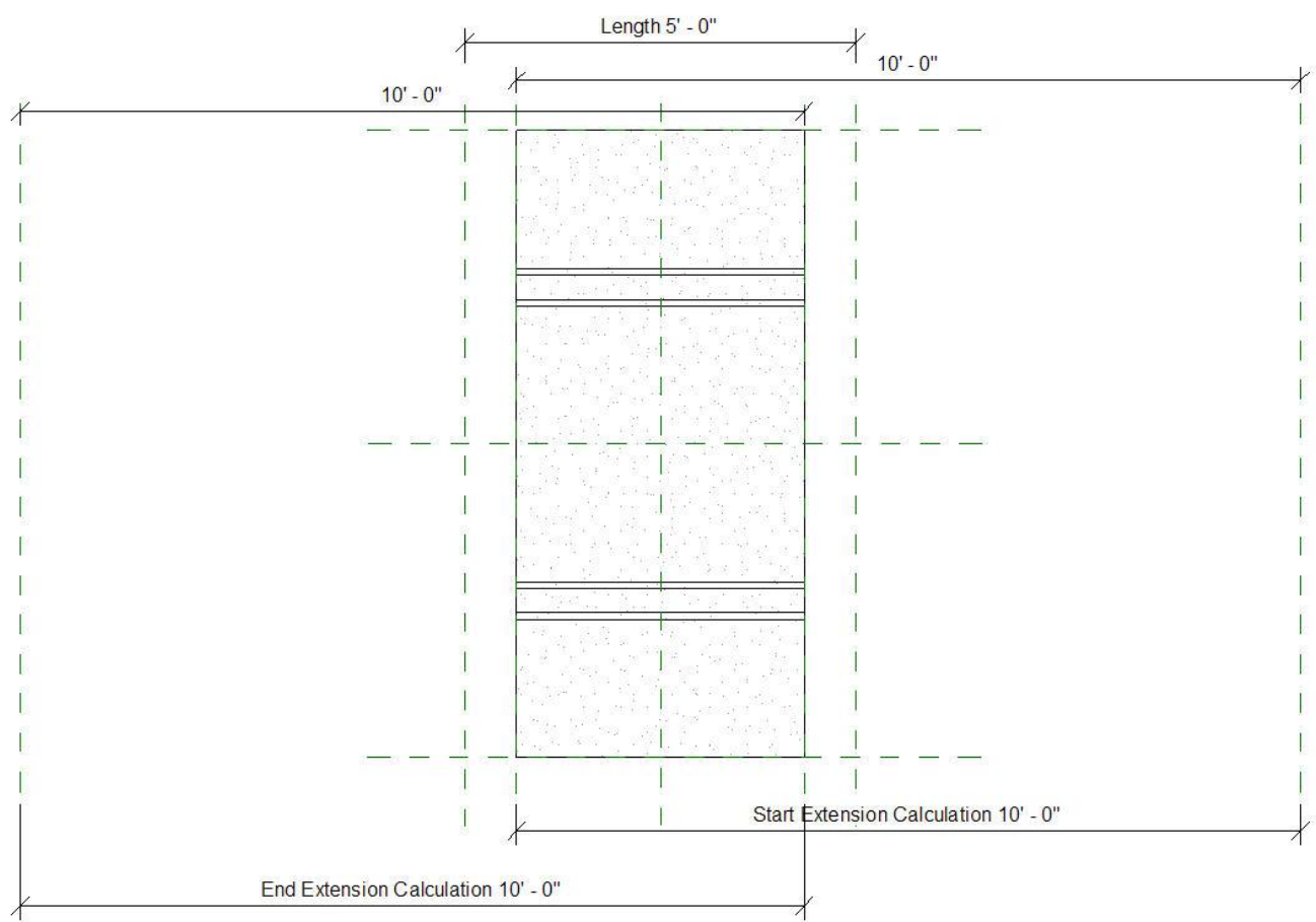
Figure 213: Precast-Double Tee
