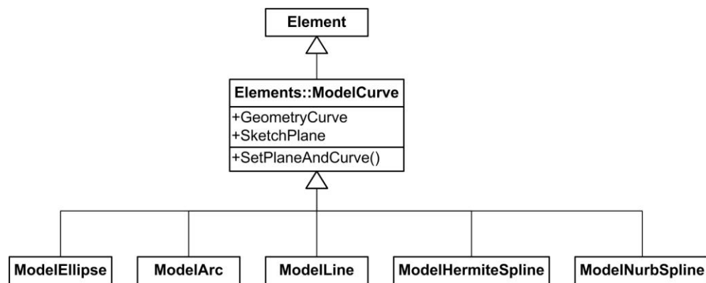
Figure 99: ModelCurve diagram
