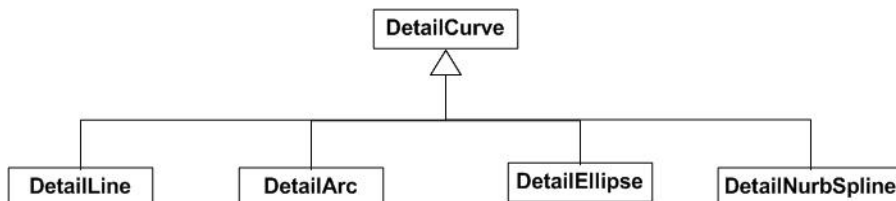
Figure 78: DetailCurve diagram
