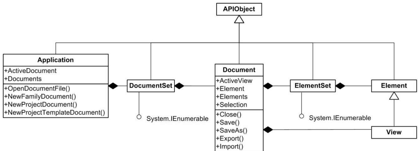
Figure 16: Application-Document-View-Element diagram
