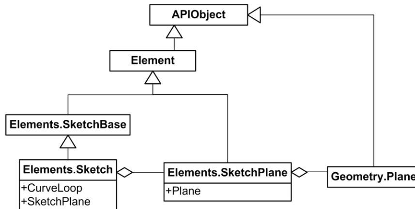
Figure 83: 2D Sketch diagram
