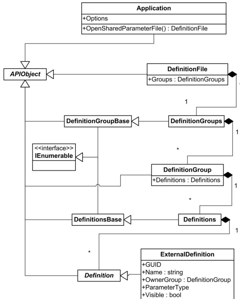
Figure 150: Get the ExternalDefinition type object diagram
