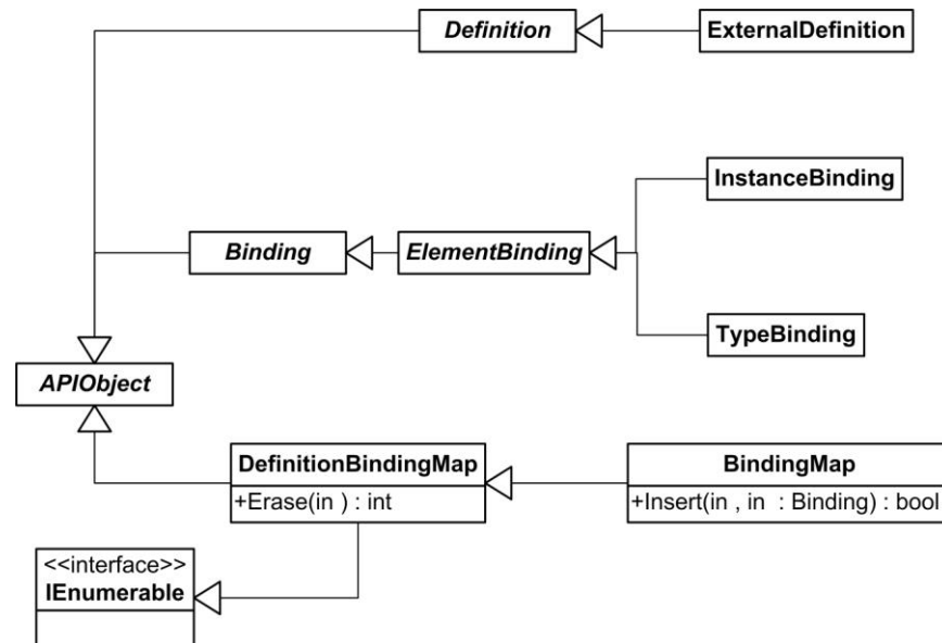
Figure 151: Binding diagram
