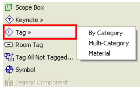
Figure 79: IndependentTag
