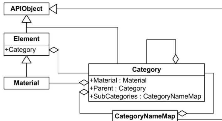
Figure 119: Material and Category diagram
